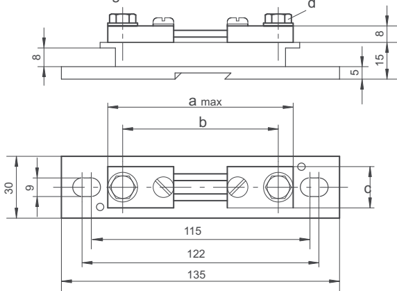
Form A with insulating base and cover
