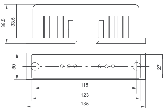
Form A with insulating base and cover
